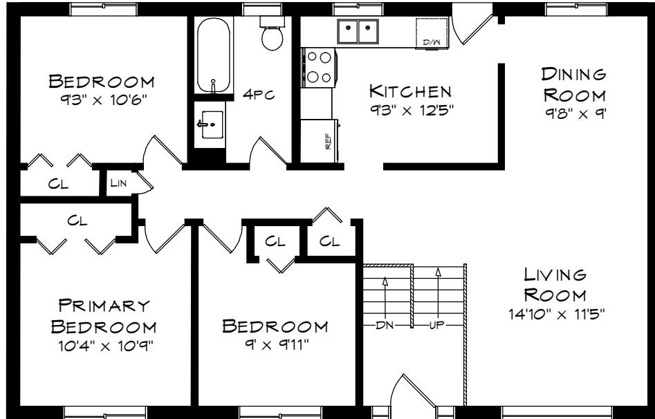
MAIN LEVEL 1,076 SQUARE FEET
