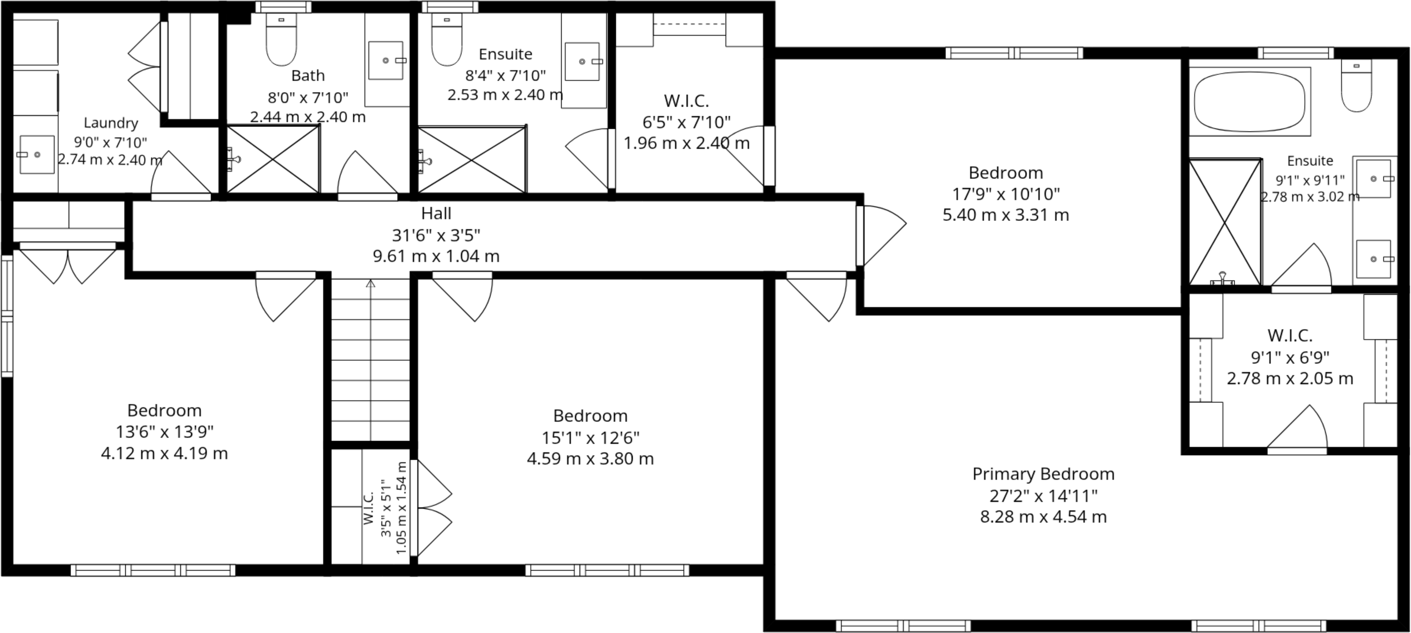
2nd Floor
